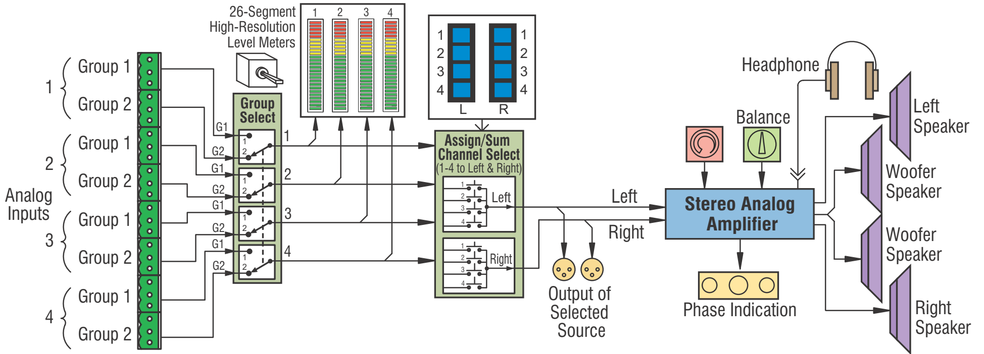
Figure 1–19 AMP2-VTR2 Block Diagram
