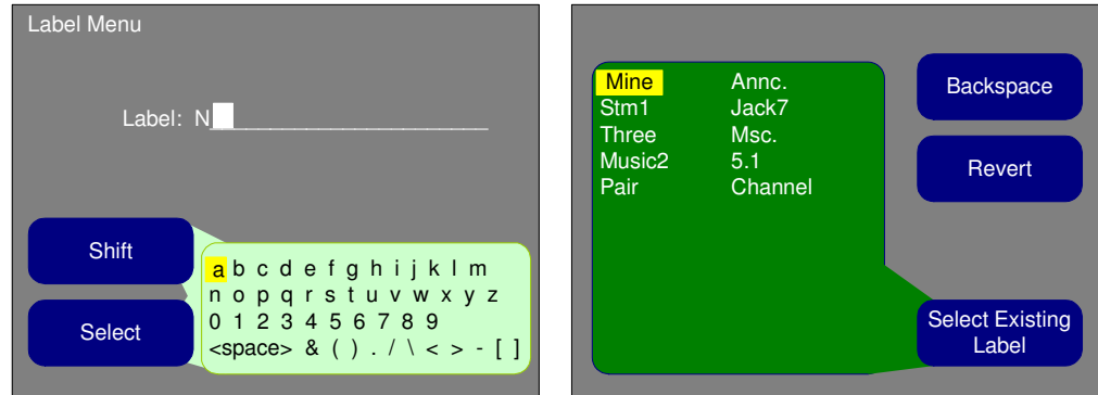
Figure 6–10 Label Menu
