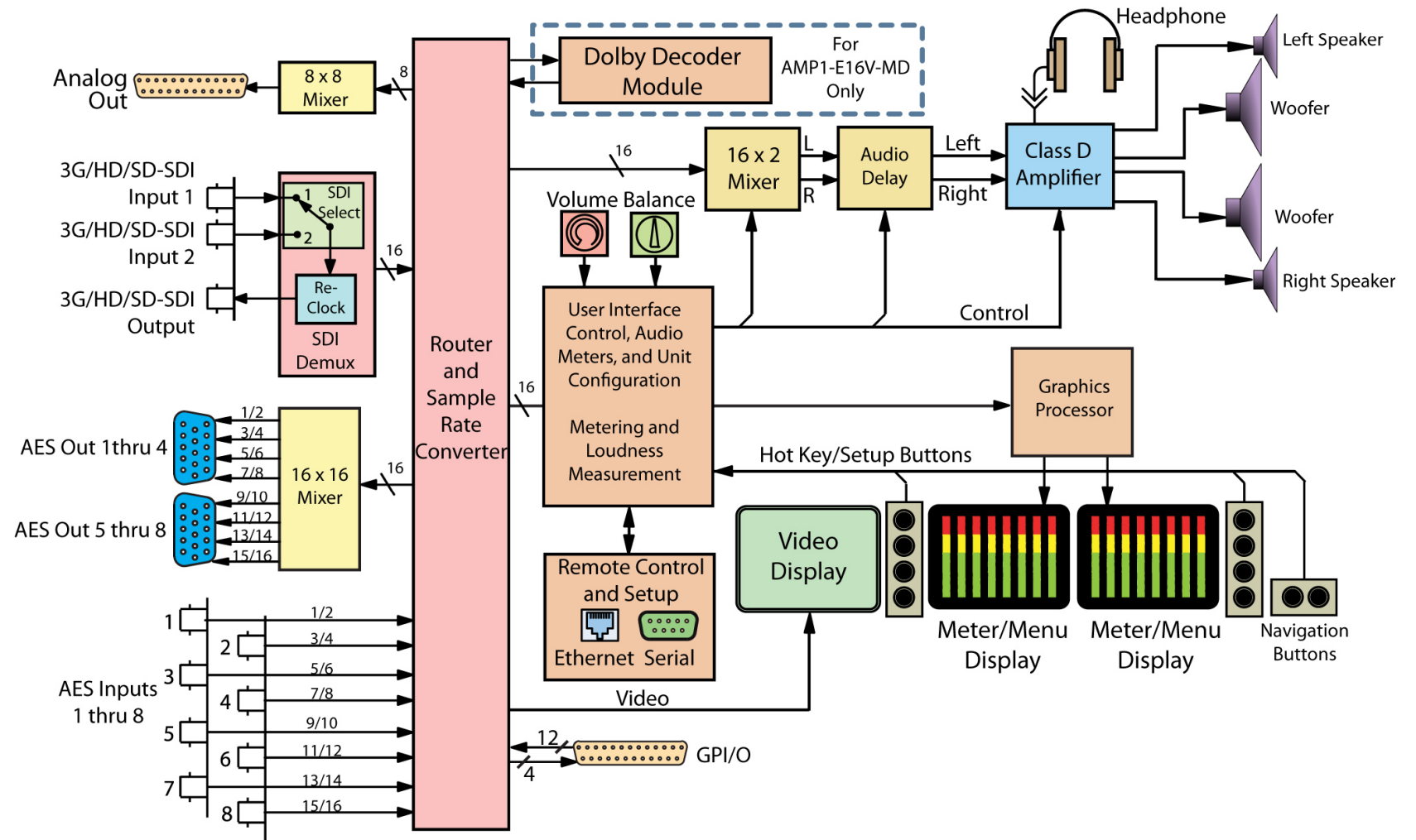
Figure 8-1 AMP1-16 Block Diagram
