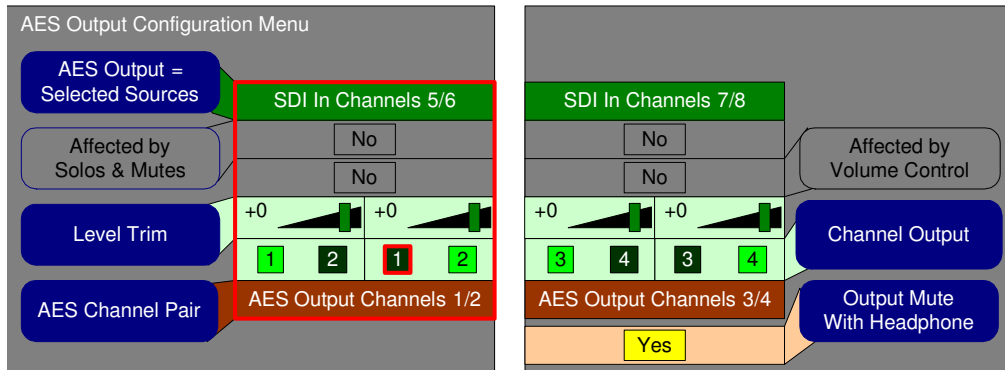
Figure 3-4 Select Outputs
