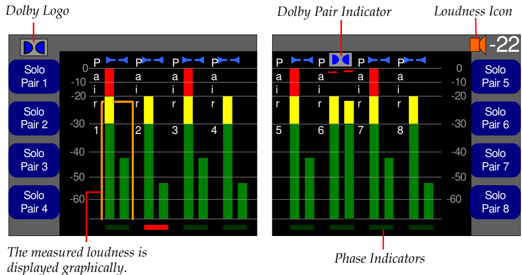
Figure 6-12 Main Screen
