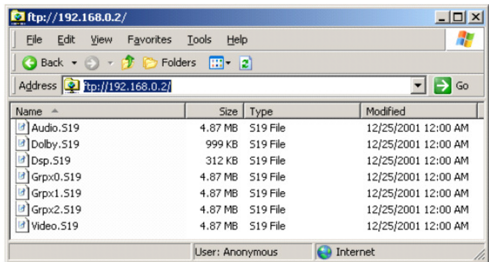
Figure 10-2 FTP Location
