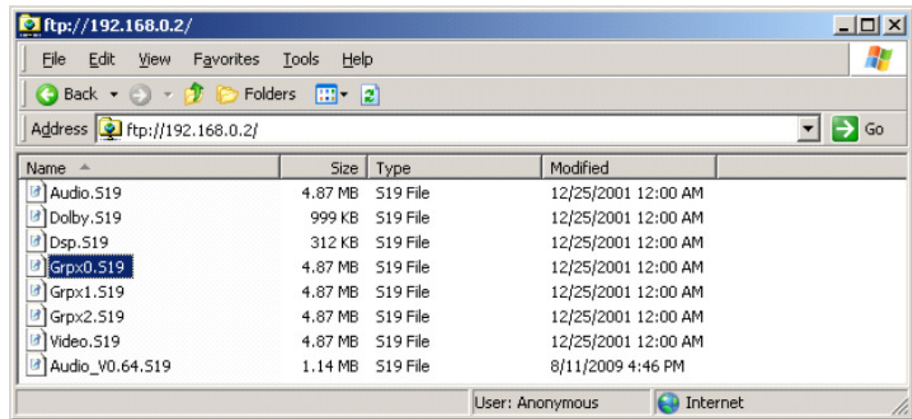
Figure 7-10 Copy Completed
