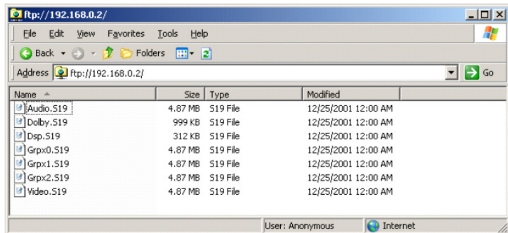
Figure 7-11 Refreshed Window
