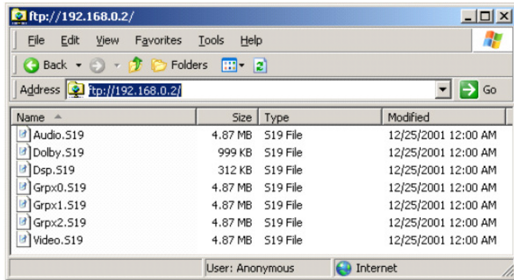
Figure 7-6 FTP Location
