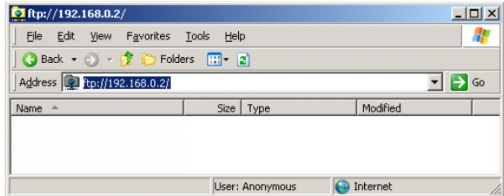
Figure 7–8 FTP Window
