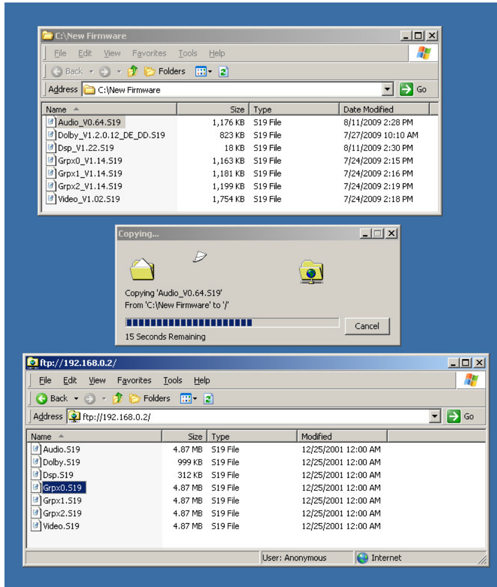
Figure 7-9 File Transfer
