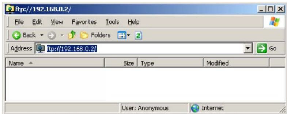
Figure 10–4 FTP Window
