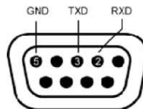
Figure 2–14 RS-232 Pin-Out
