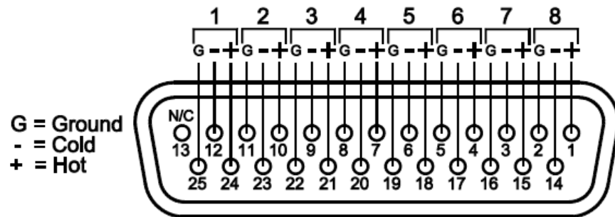
Figure 2-9 Analog Input Connector Pin-Out
