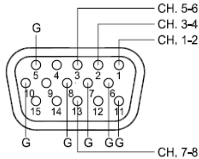
Figure 2-11 AES Unbalanced Out from SDI HD-15 Pin-Out
