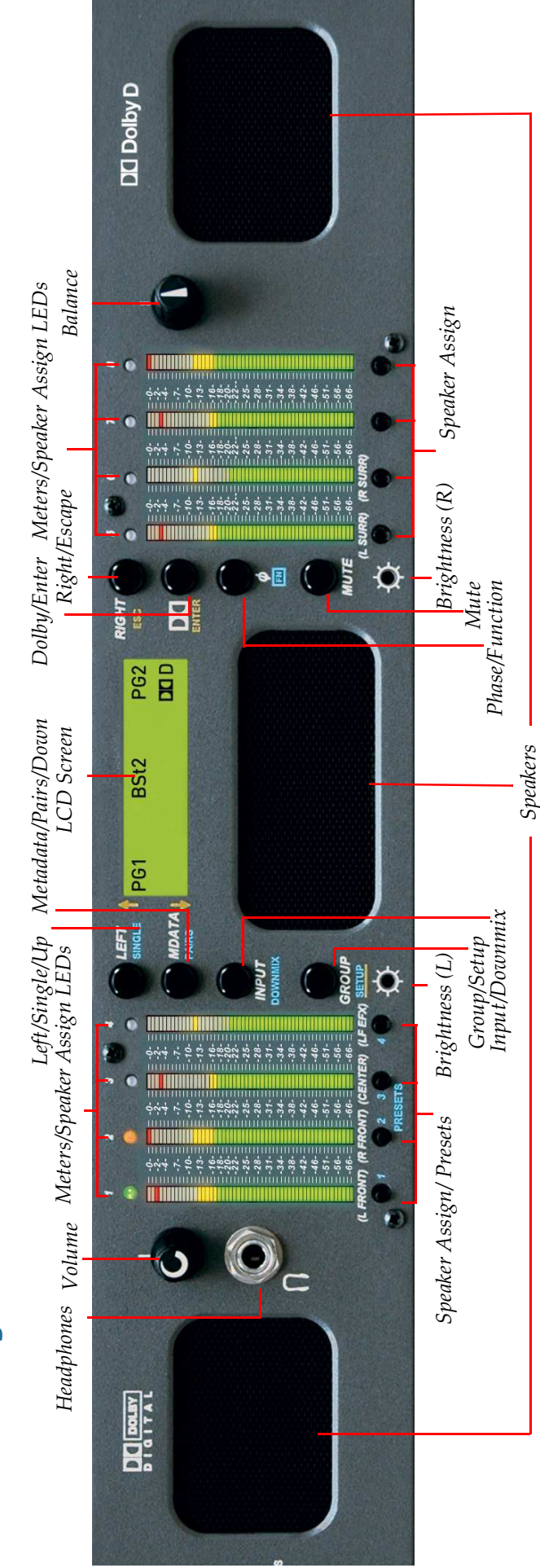
Figure 2-2 The AMP2-D8 Series Front Panel
