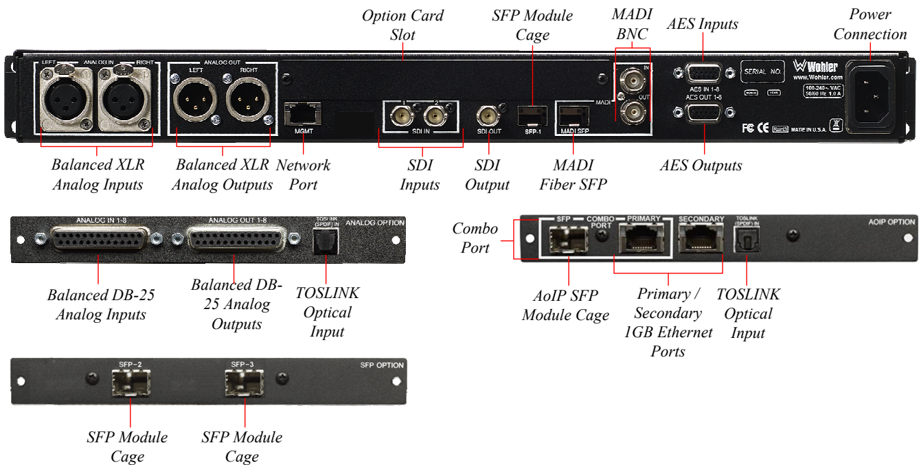
Figure 2-2: iVAM1-3 Rear Panel & Option Cards
