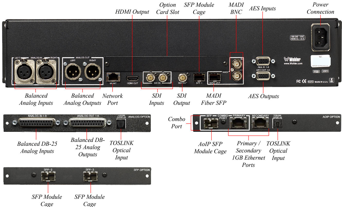
Figure 2-2: iVAM2-2 Rear Panel & Option Cards
