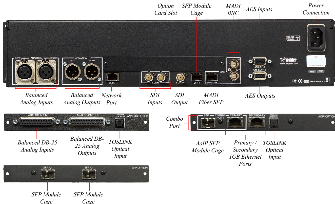
Figure 2-2: iAM-AUDIO-2 PLUS Rear Panel & Option Cards
