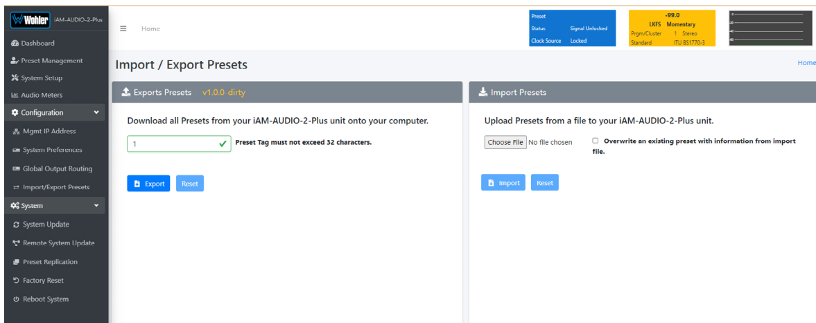
Figure 4-23: Database Export
