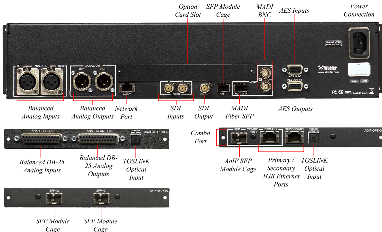
Figure 2-2: iAM2-8 Rear Panel & Option Cards
