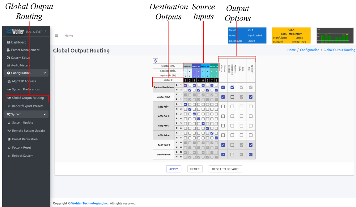
Figure 4-20: Global Output Routing Option
