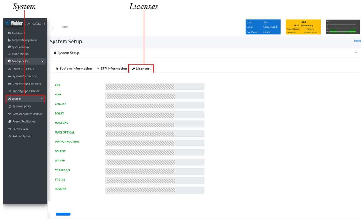
Figure 4-28: Licenses Tab
