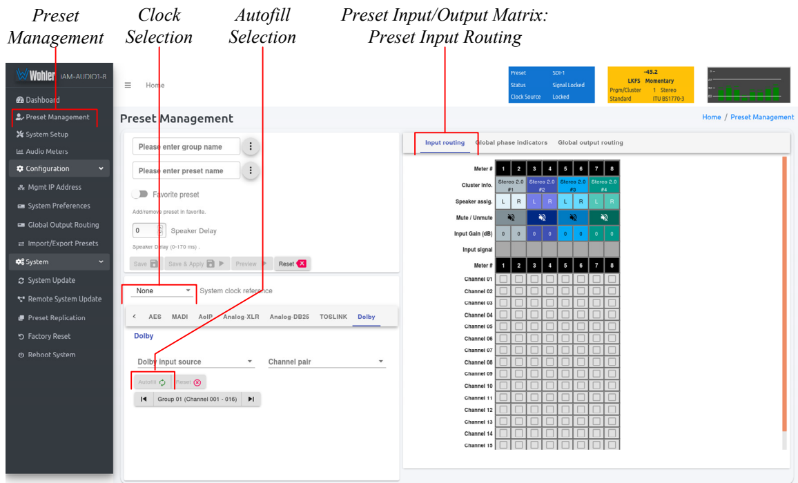
Figure 4-15: Configure Presets
