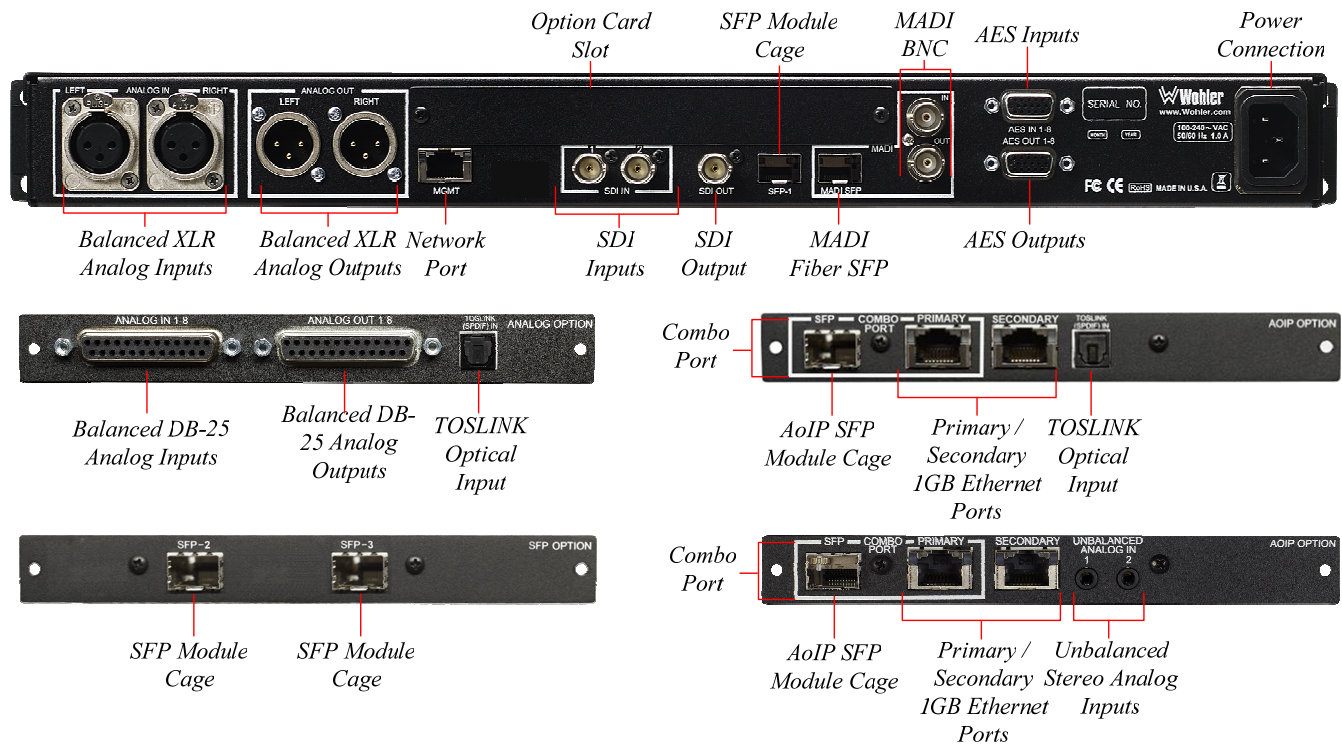
Figure 2-2: iAM1-8 Rear Panel & Option Cards
