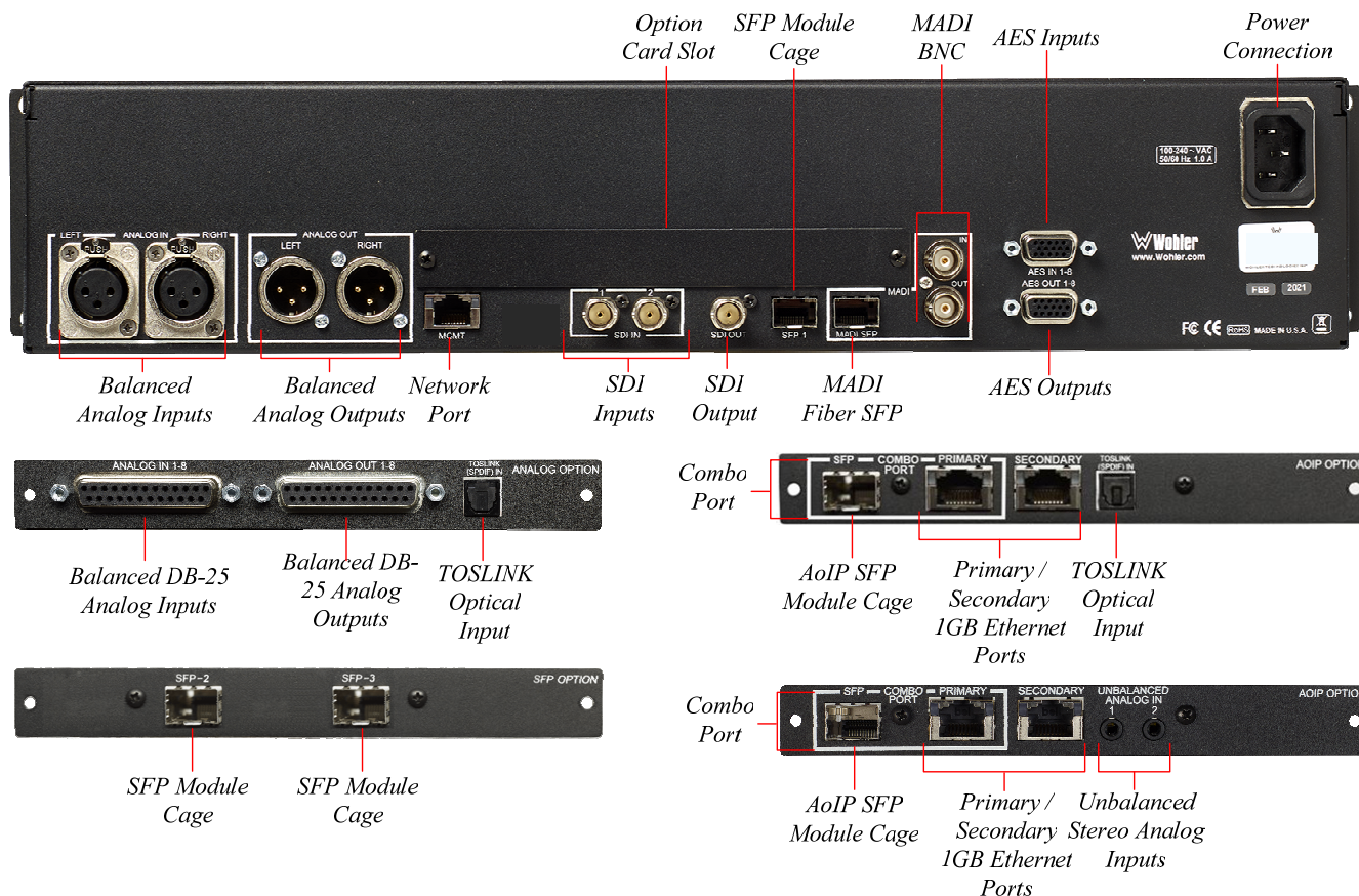
Figure 2-2: iAM-AUDIO-2 PLUS Rear Panel & Option Cards
