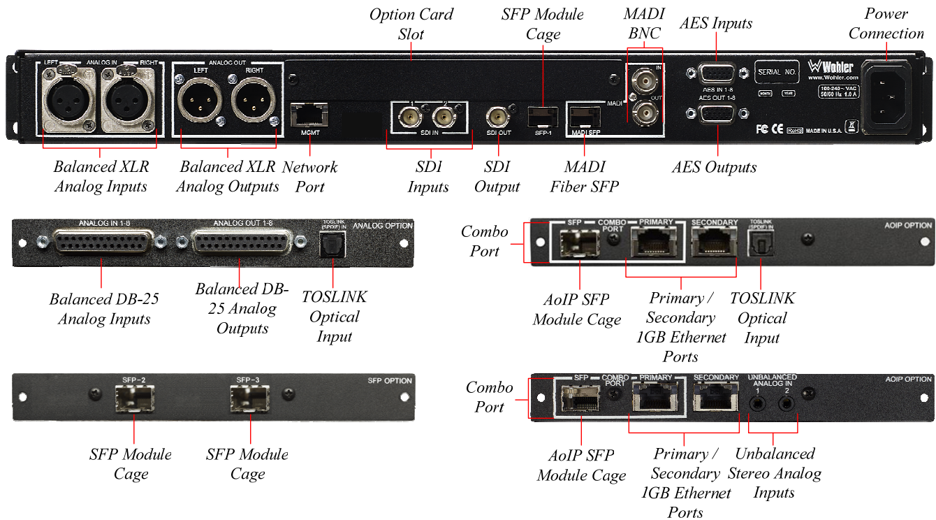
Figure 2-2: iAM-SUM Rear Panel & Option Cards
