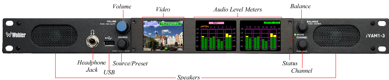
Figure 2-1: iVAM1-3 Front Panel
