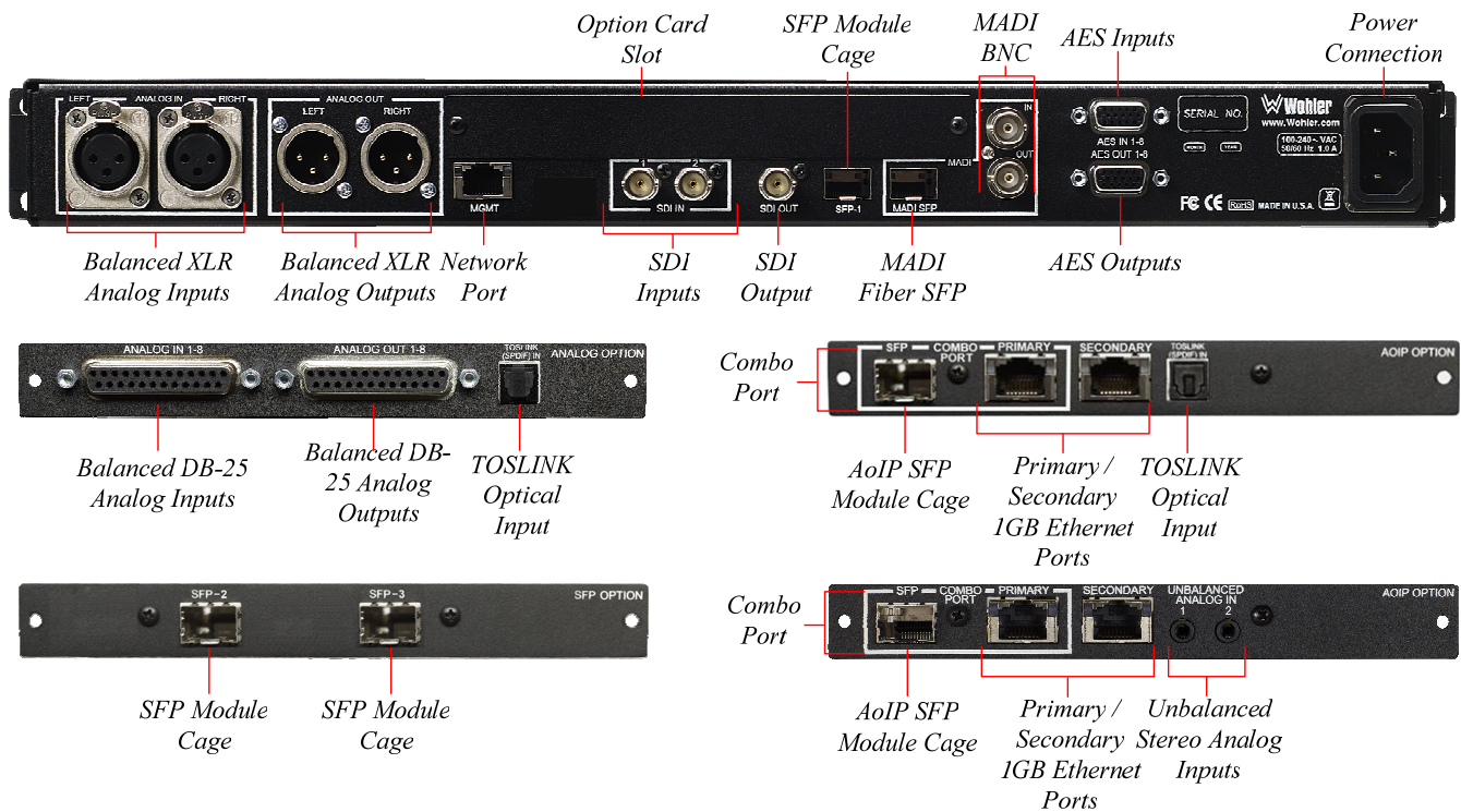
Figure 2-2: iVAM1-3 Rear Panel & Option Cards
