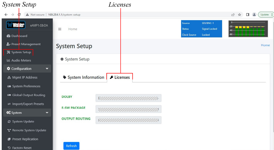
Figure 4-23: Licenses Tab
