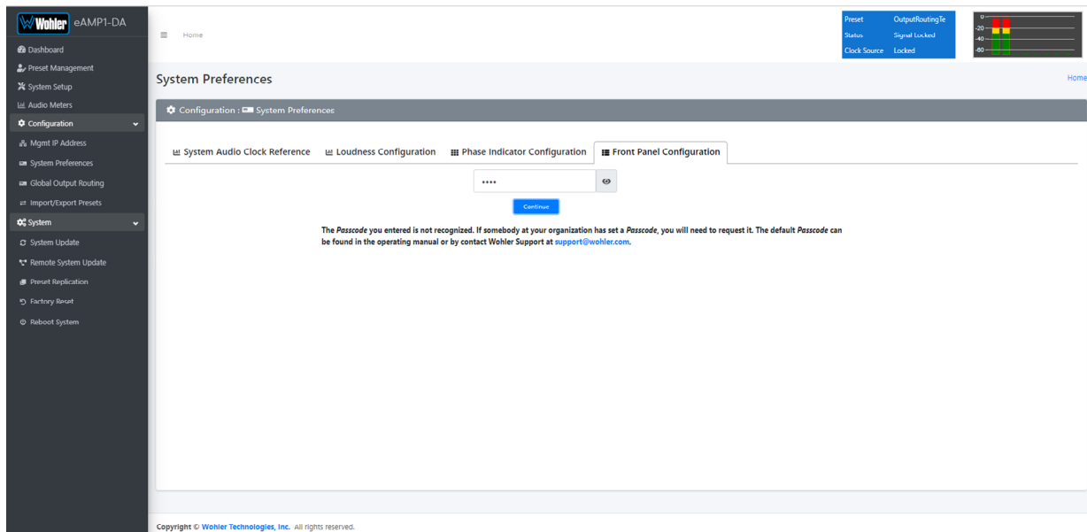
Figure 4-12: Unrecognized Passcode
