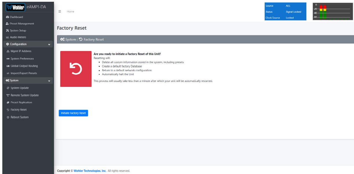
Figure 4–24: Factory Reset
