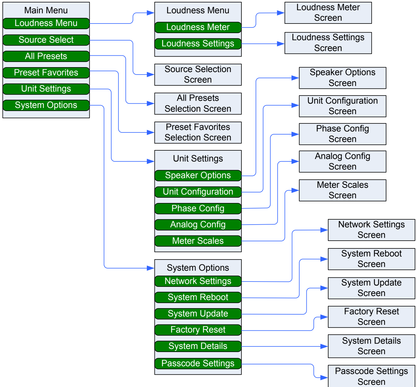
Figure 2-7: Menu Tree
