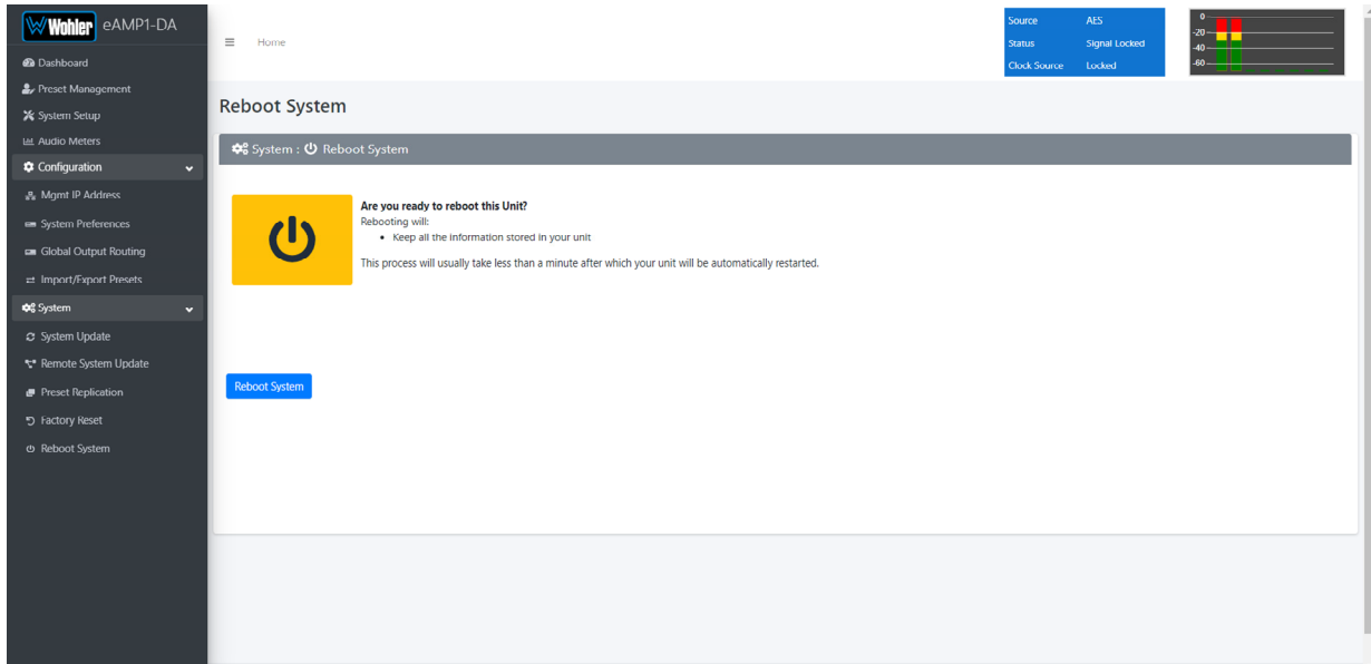
Figure 4-25: Reboot System
