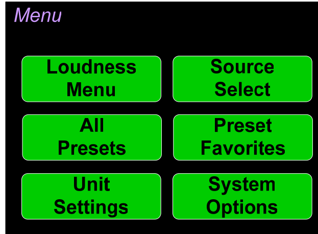
Figure 2-8: Main Menu
