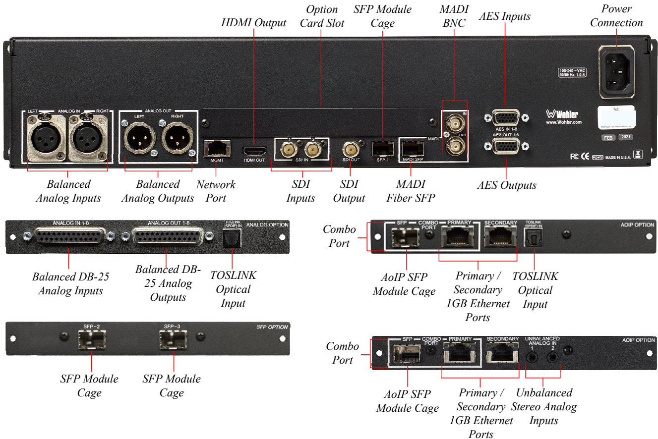
Figure 2-2: iVAM2-12G Rear Panel & Option Cards
