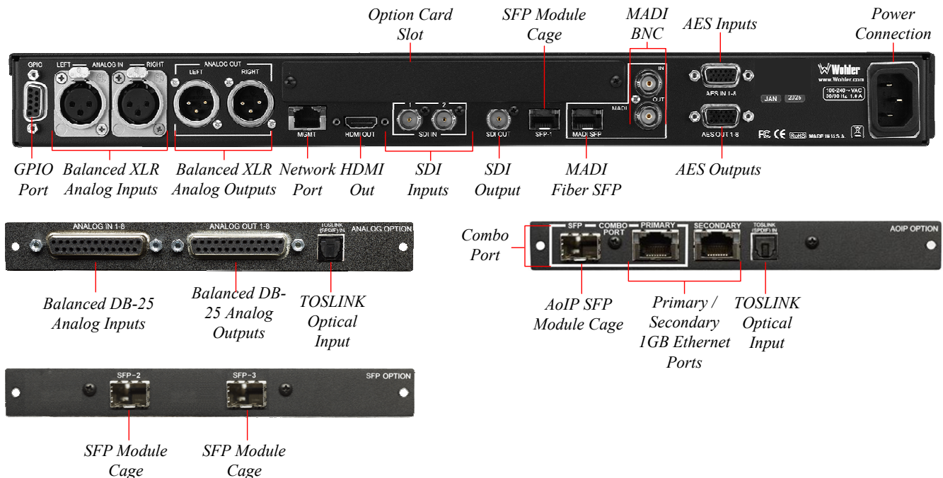
Figure 2-2: iVAM1-SUM16-G Rear Panel & Option Cards
