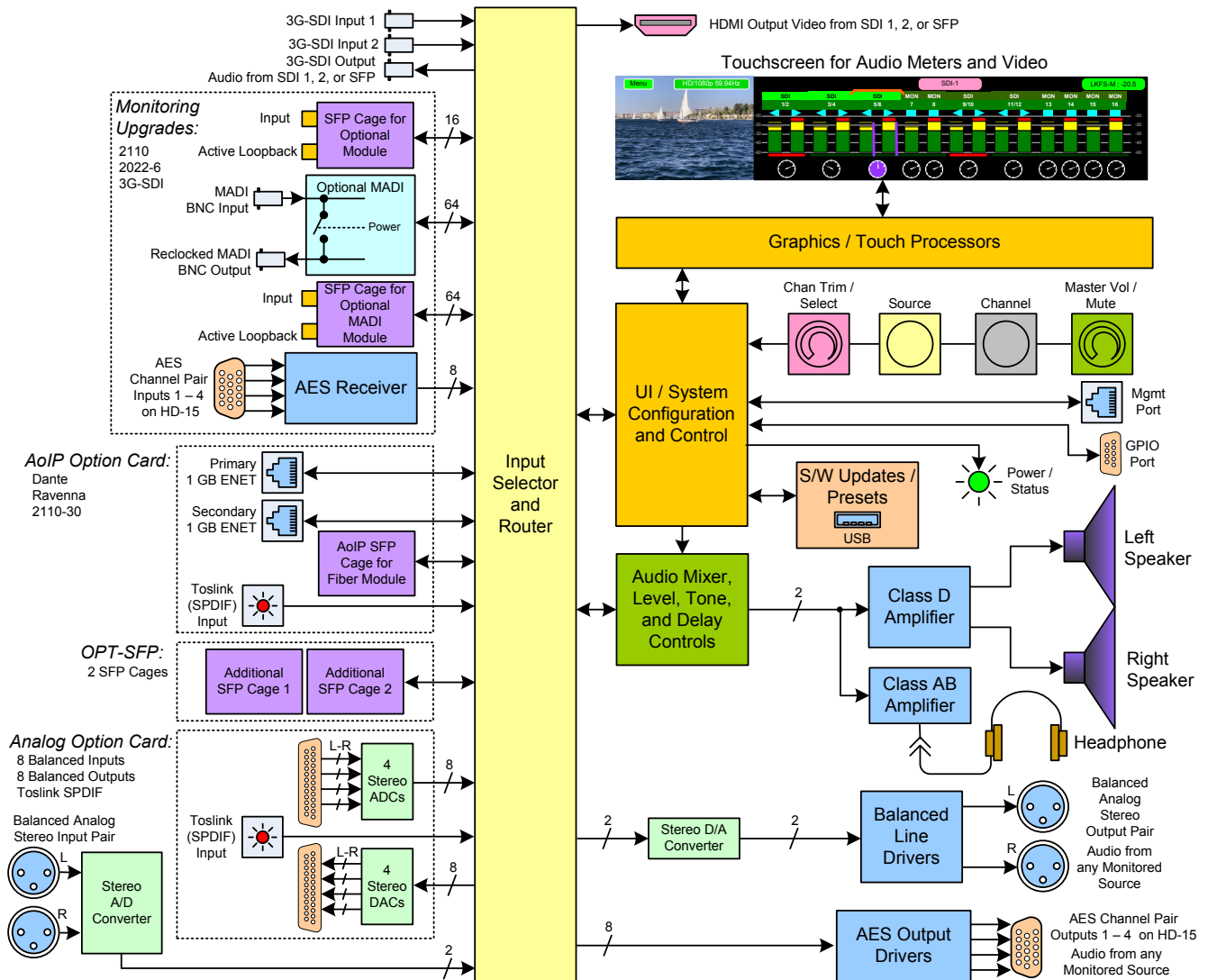
Figure 3-1: /VAM1-SUM16-G Block Diagram
