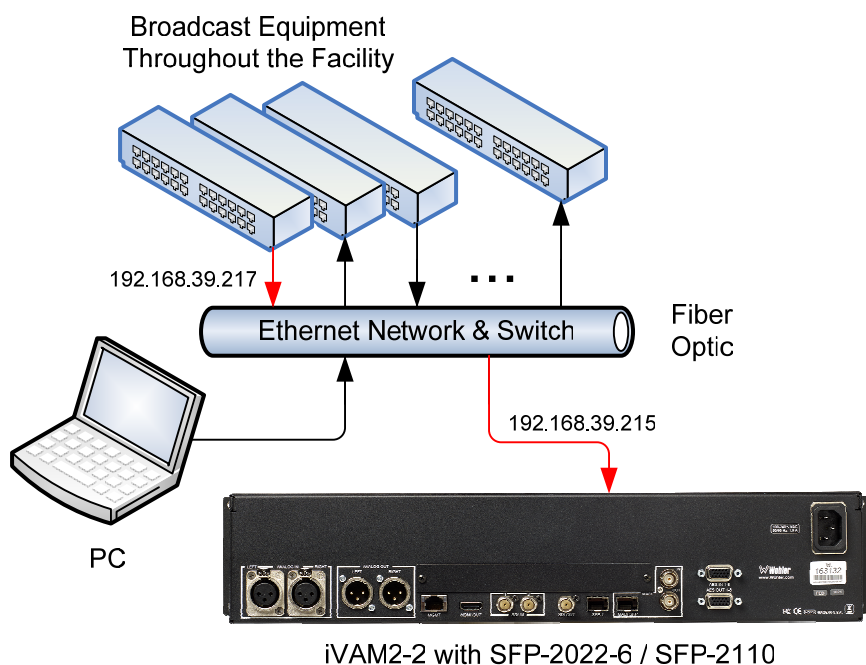
Figure 2-8: SFP-2022-6 and SFP2110 Network Diagram
