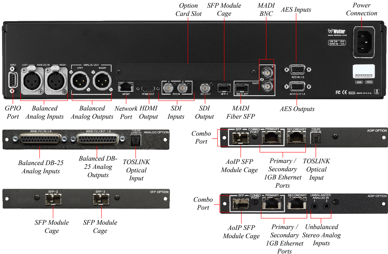
Figure 2-2: iVAM2-2-G Rear Panel & Option Cards
