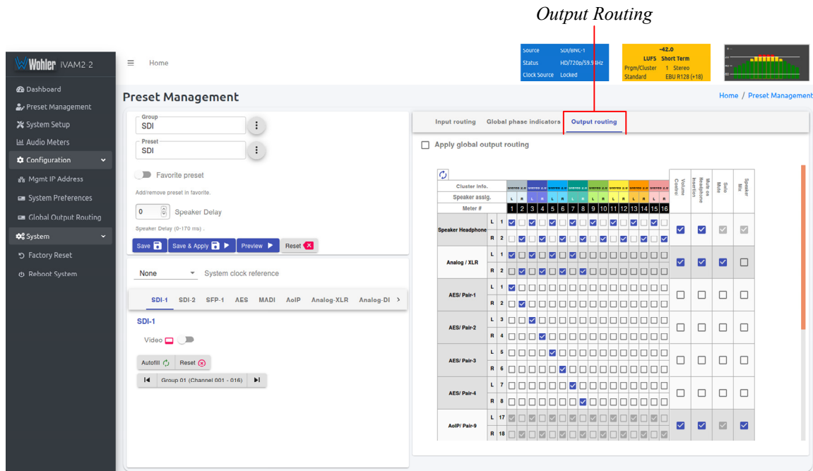
Figure 4-19: Output Routing Preset Tab
