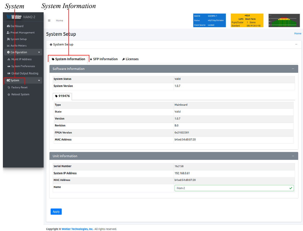
Figure 4-27: System Information Tab
