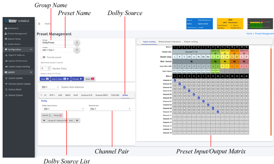
Figure 4-20: Creating a Dolby Preset
