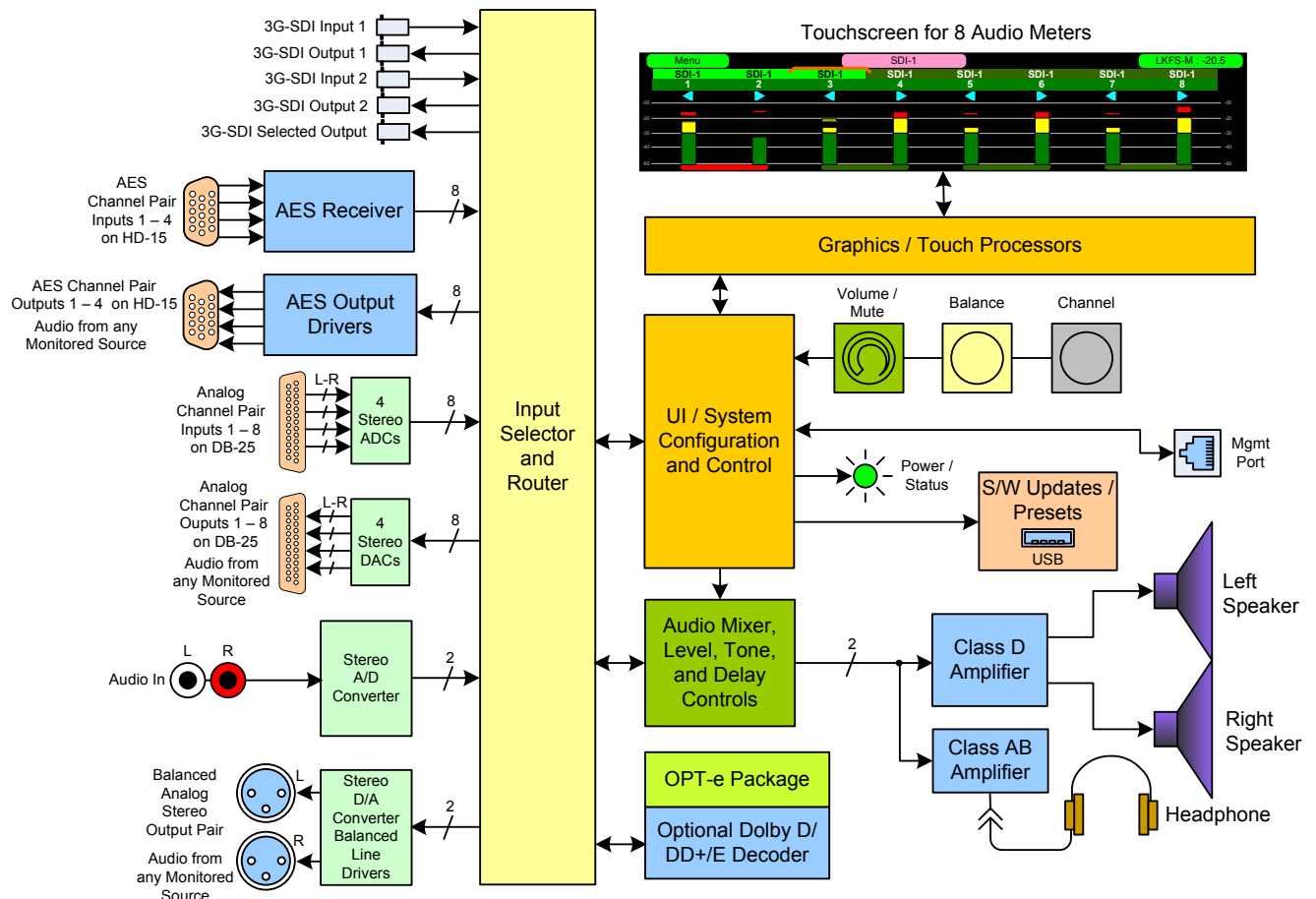
Figure 3-1: eAMP1-S8-2MDA Block Diagram
