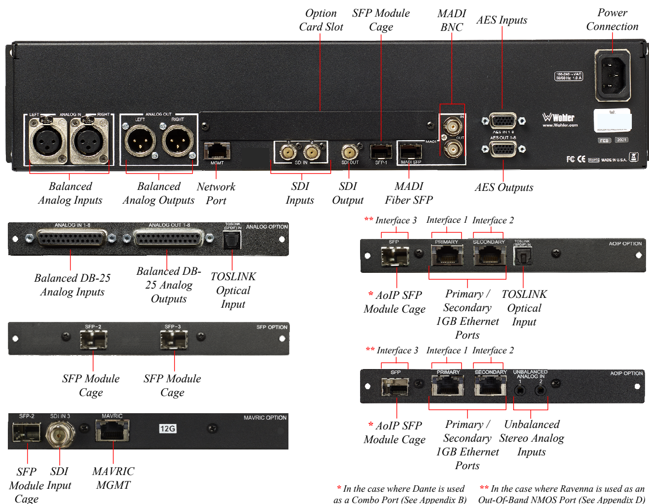
Figure 2-2: iAM-AUDIO-2 PLUS Rear Panel & Option Cards
